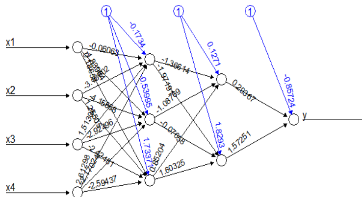
Fig. 2. The architecture of the MLFF neural network with four input variables, two hidden layers and one output node
